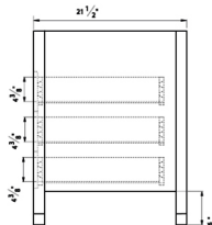
SIDE
